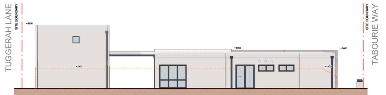
West Elevation
