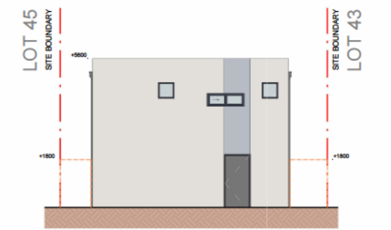
Garage South Elevation
