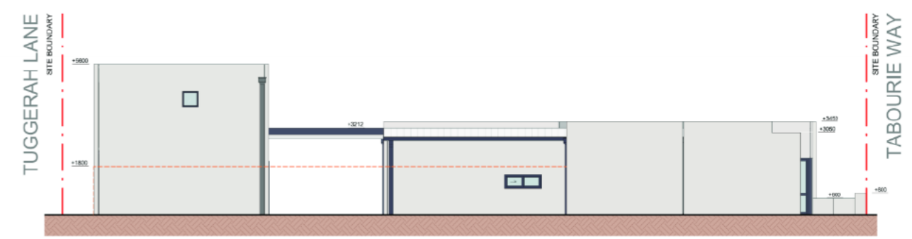
Left Elevation
